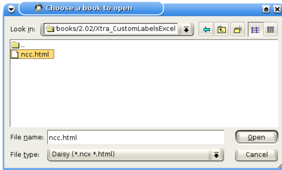
Figure 2: Daisygui screenshot.
